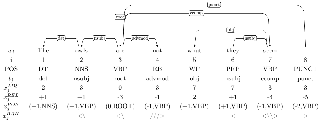
Figure 2: Encoding of a given dependency tree with the x_j field encoded according to the naive absolute, naive relative, POS-based, and bracketing-based encodings.
